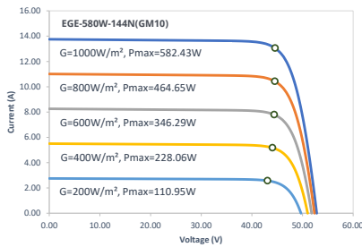
IV-Curves Irradiance
