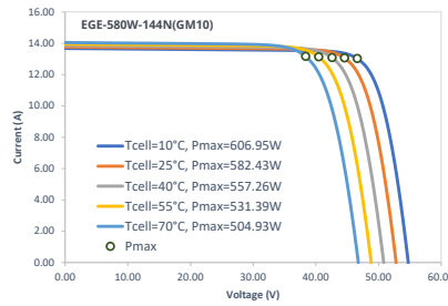
IV-Curves Temperature
